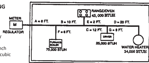
Low Pressure (5" to 7" WC) Natural Gas (Series System)
