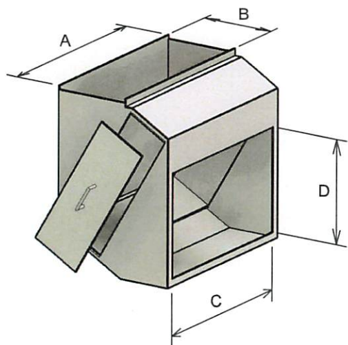
ALTERAIRE BOOT WITH COVER
