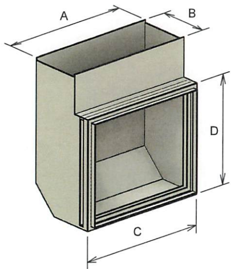
COMPACT RETURN AIR BOOT
